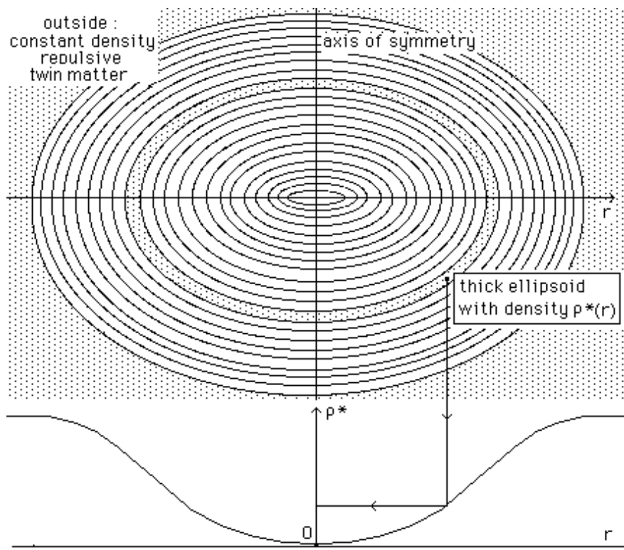
Fig. 5: Ad hoc twin matter distribution, for 3d confinement. The density is constant between successive homothetic flat ellipsoids.
