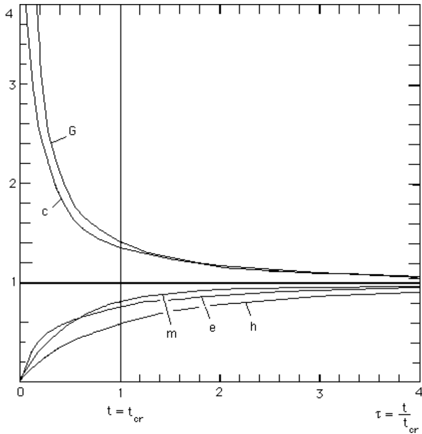
Fig. 16: Variation of the constants during the radiative era. \tau \gg \tau_{cr} corresponds to matter era
