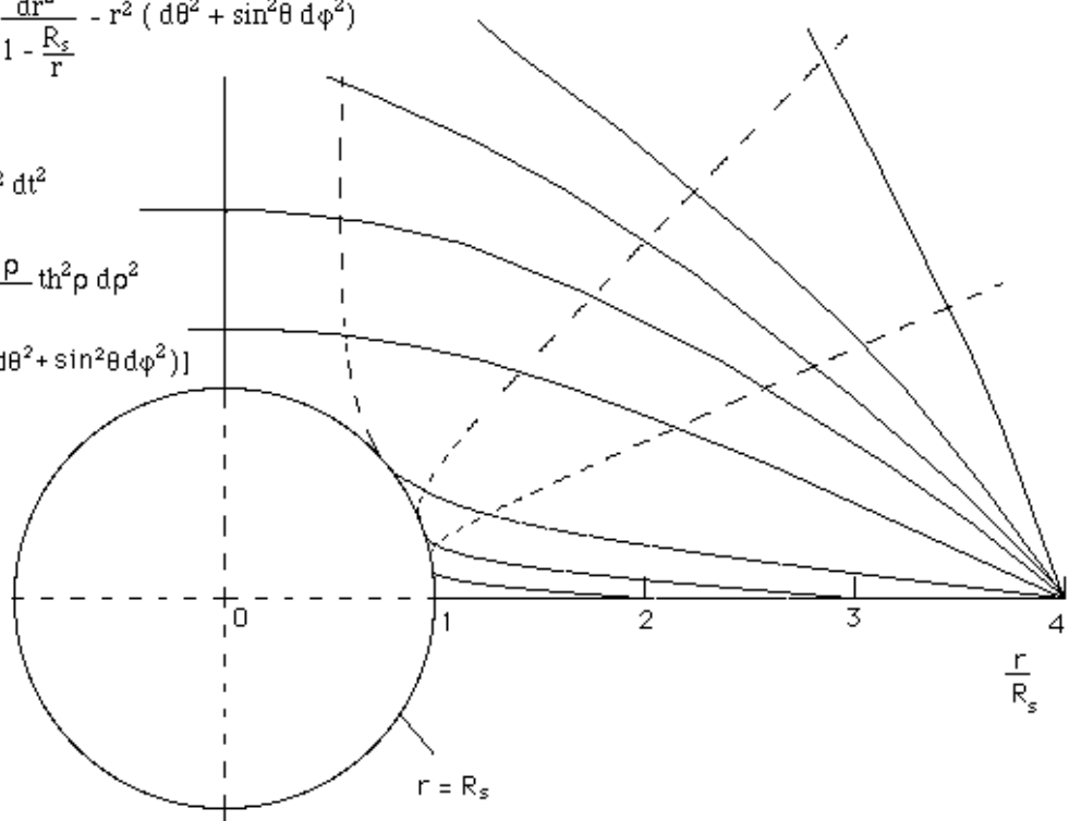
Fig. 26: 3d metric hypersurface with a “space bridge”. Geodesics.
