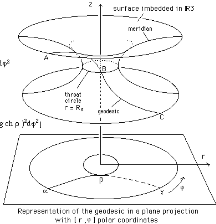
Fig. 25: 2d metric of a surface with a "bridge" linking two folds.
