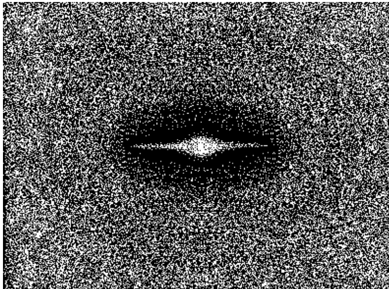
Fig. 7: The galaxy, plus its environment of hot twin matter.
