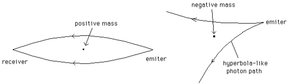
Fig. 10-a: Positive gravitational lensing effect
