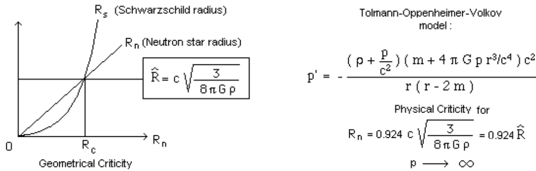
Fig. 22: Left, geometrical criticality. Right: physical criticality.
